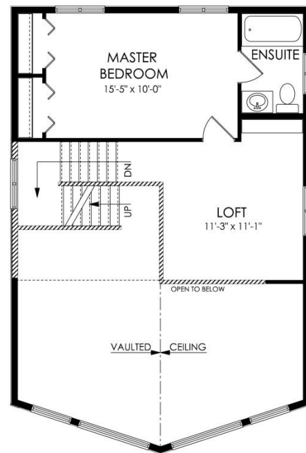
UPPER FLOOR PLAN - 410 SQ. FT.
